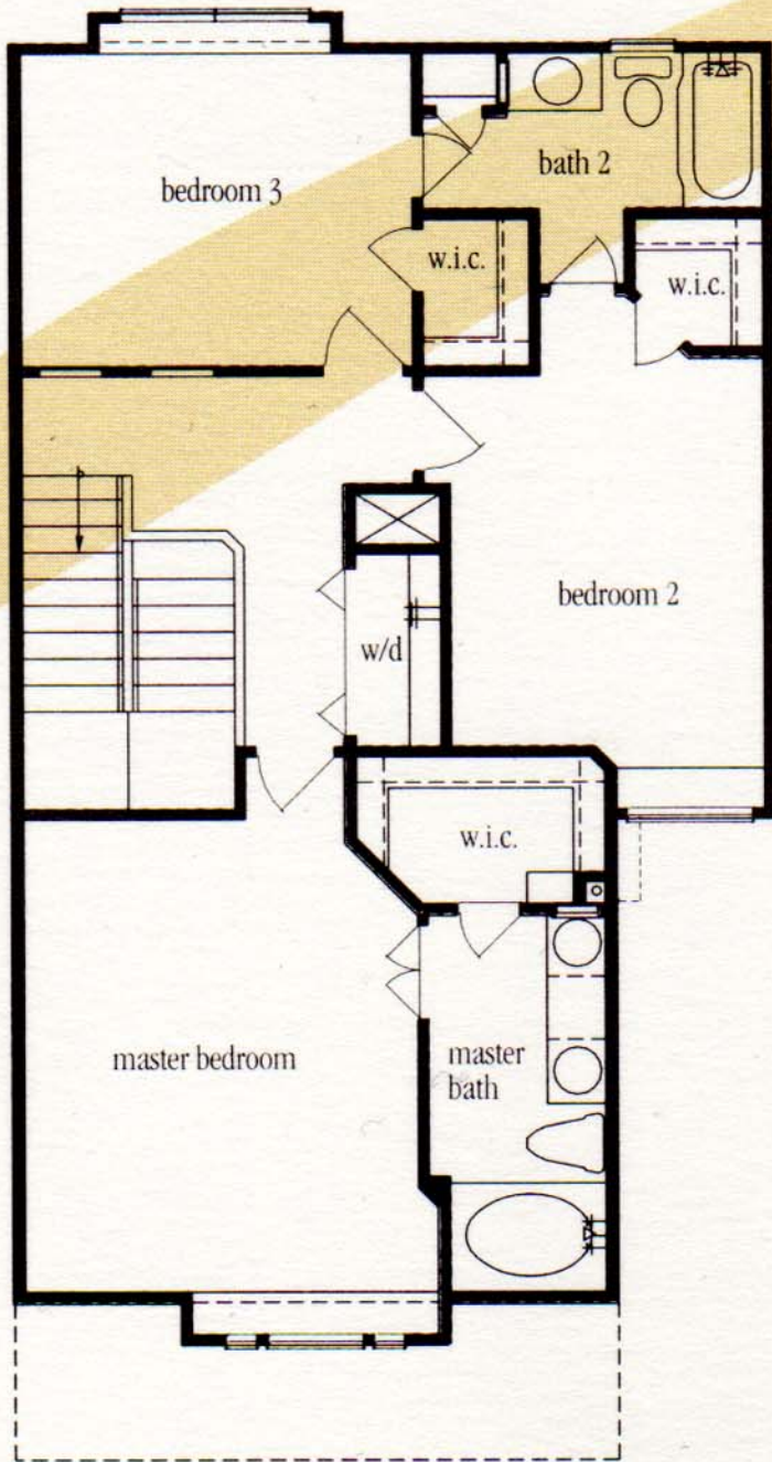
second floor
